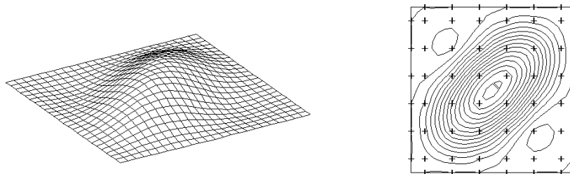
Figure 17. First buckling mode of a clamped square plate under pure shear. Result generated using 6x6 constant domain cells inside the domain, and 26 constant boundary elements.
