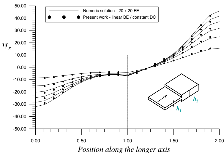
Figure 19. Non-linear results for non-null rotation along the central line for the case illustrated in Fig.18.
