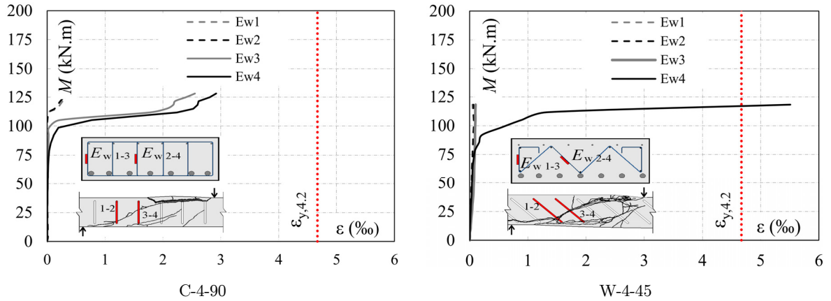
Figure 13: Strains on the shear reinforcement.
