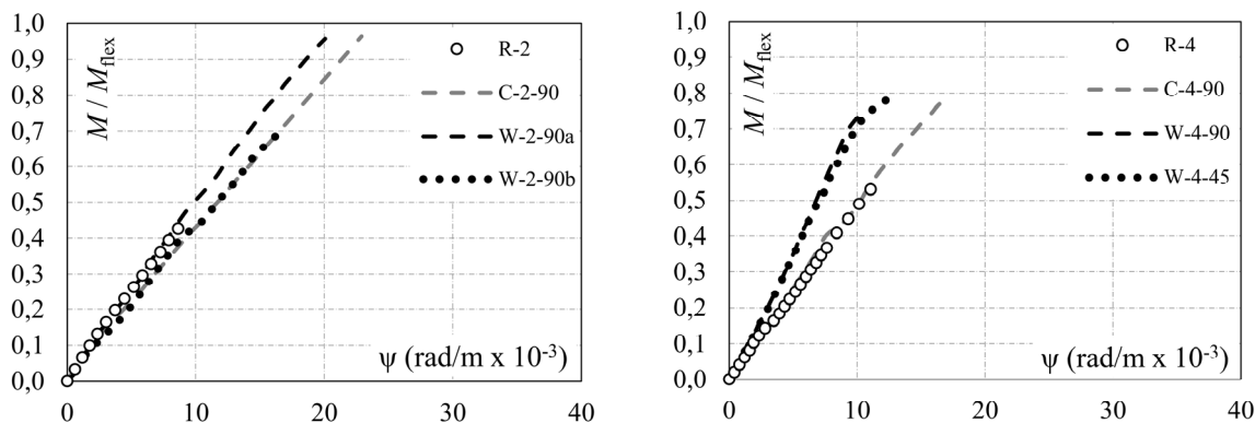
Figure 11: Flexural response of tested specimens.
