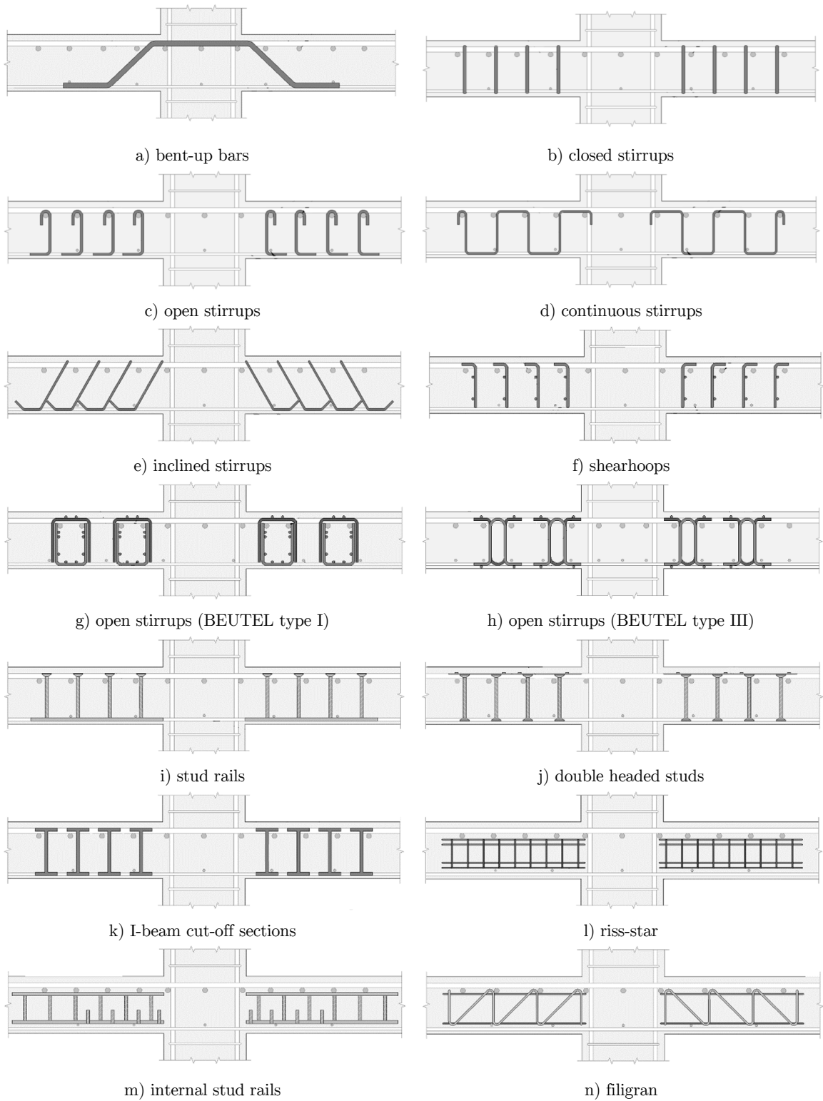
Figure 4: Types of shear reinforcement for flat slabs.
