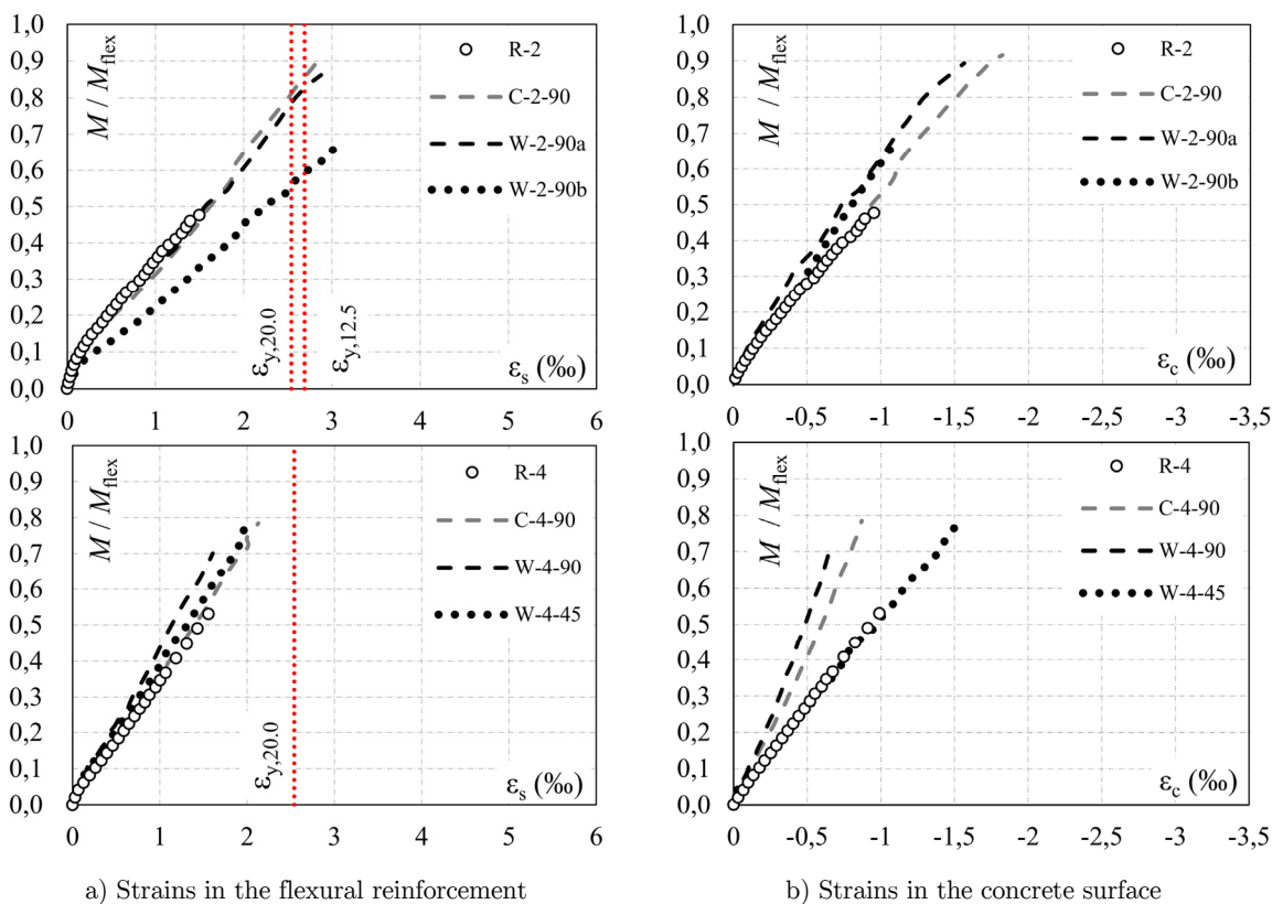
a) Strains in the flexural reinforcement
