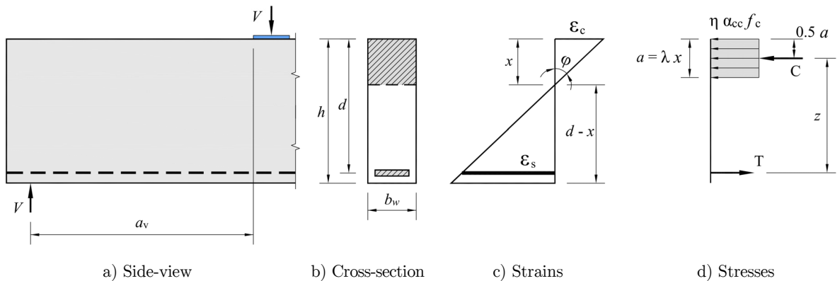
Figure 7: Assumed strain and stresses distribution in the ultimate limit state.
