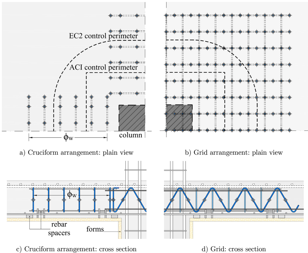
Figure 3: Arrangements of “W” stirrups in slab-column connections.
