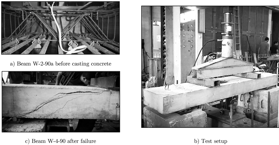
Figure 9: Photos of different stages of the experimental program.
