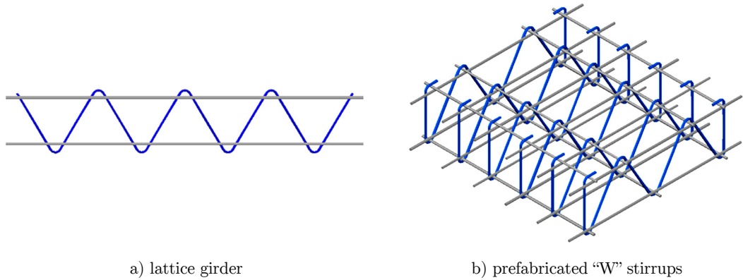
Figure 2: Prefabricated cage of “W” stirrups.
