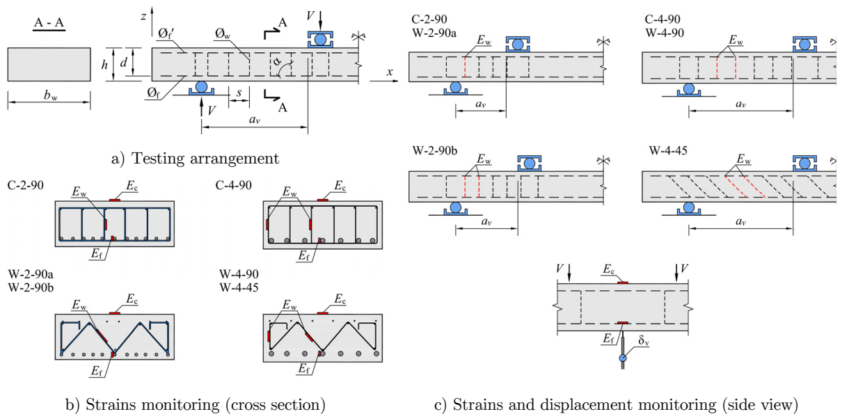
Figure 8: Illustration of the testing system and of monitoring of strains and displacements.
