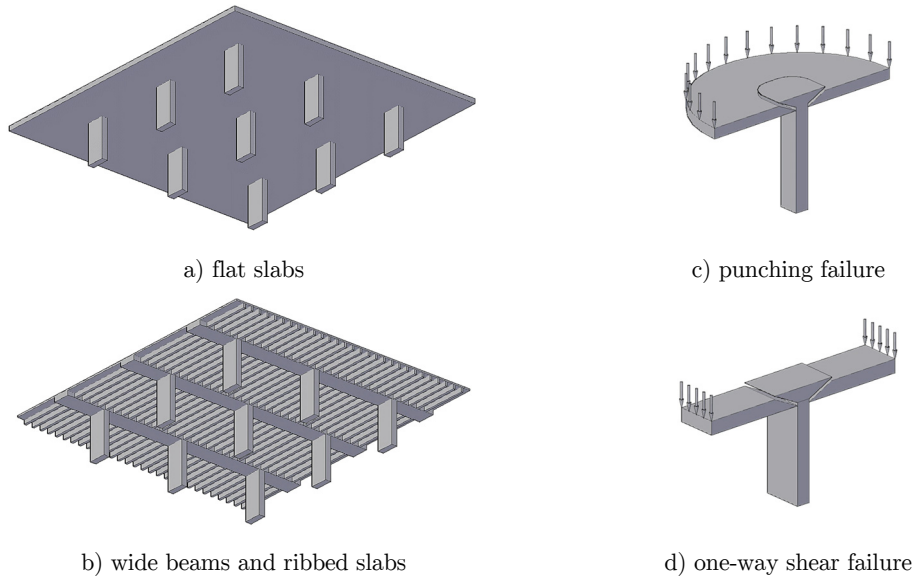
Figure 1: Shear failure of flat flooring systems
