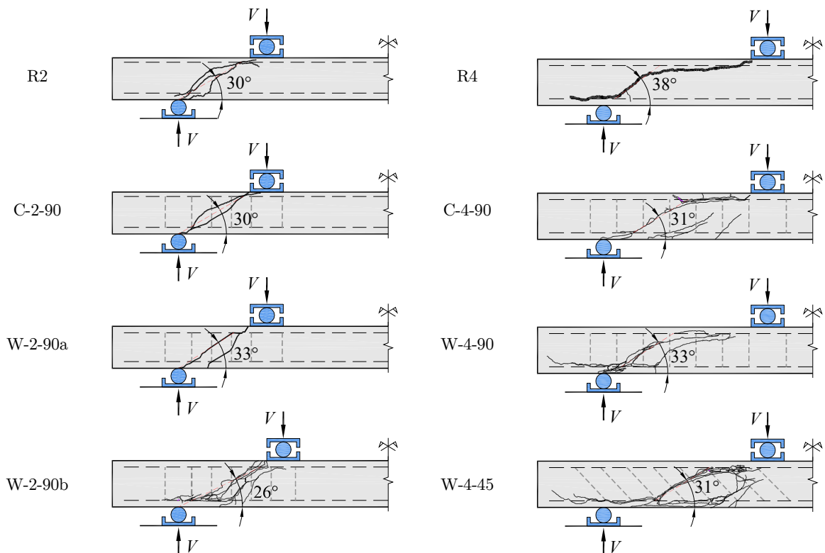
Figure 10: Cracking pattern after failure.
