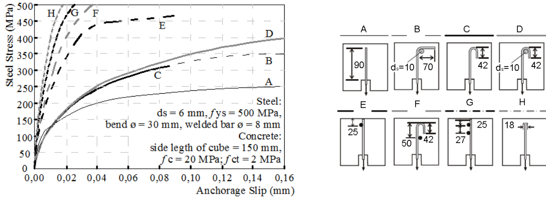
Figure 6: Computational analysis of different anchorage types (Beutel and Hegger, 2002).
