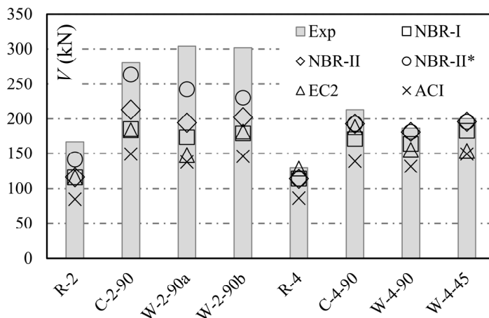
Figure 14: Comparison between experimental and theoretical results.
