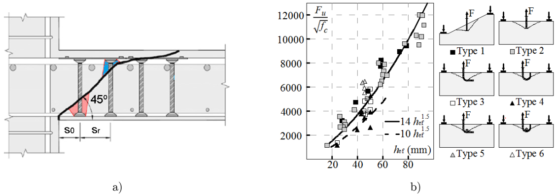
Figure 5: a) Different anchorage conditions in a slab-column connection. b) Pull out resistance of tensioned bars (Regan, 2000).
