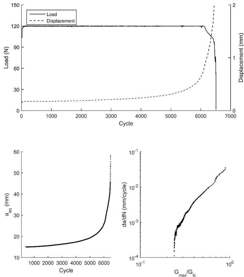
Figure 4: Example of experimental fatigue test: raw load-displacement data direct from machine (top), equivalent crack length as a function of cycles (bottom left), and respective Paris Law representation (bottom right).
