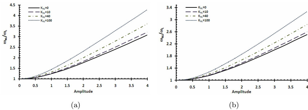
Figure 6 The effect of the nonlinear stiffness K_{NL} on the nonlinear to the linear frequency ratio (Left) Simply supported, (Right) Fixed-Fixed boundary conditions
