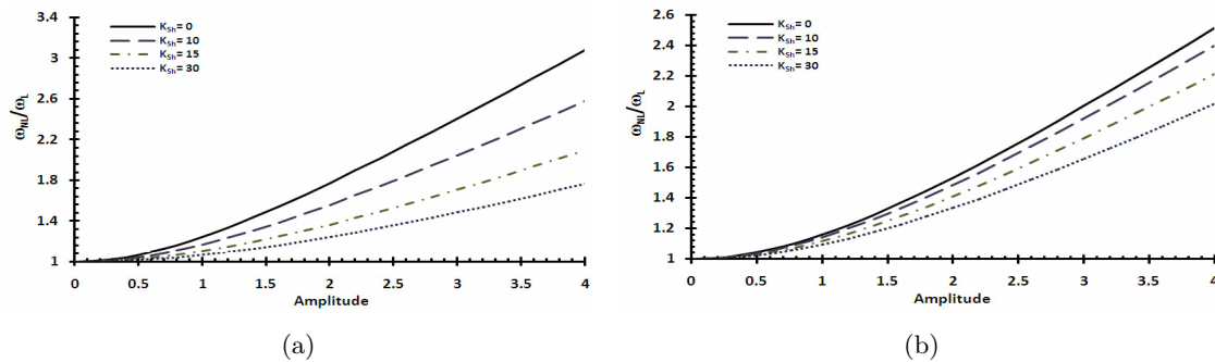
Figure 7 The effect of the shear stiffness K_{Sh} on the nonlinear to the linear frequency ratio (Left) Simply supported, (Right) Fixed-Fixed boundary conditions
