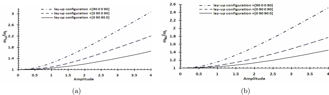
Figure 3 The effect of cross-ply lay-up configuration on the nonlinear to the linear frequency ratio (Left) Simply supported, (Right) Fixed-Fixed boundary conditions
