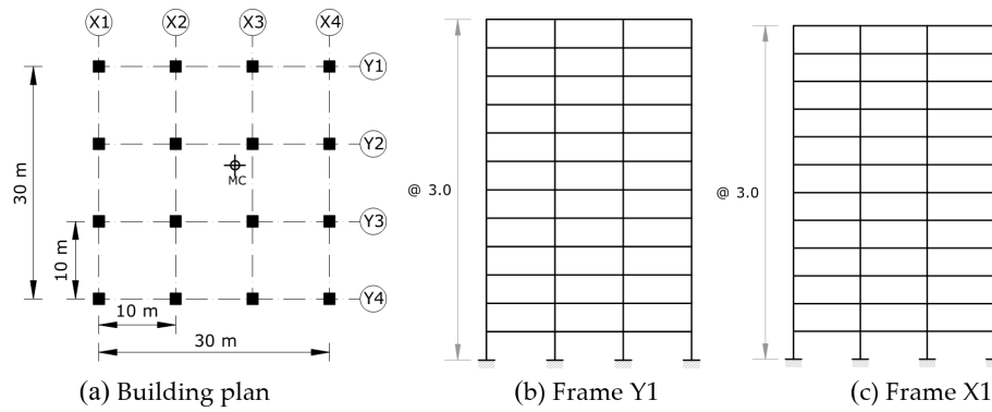
Figure 7 12-story building.
