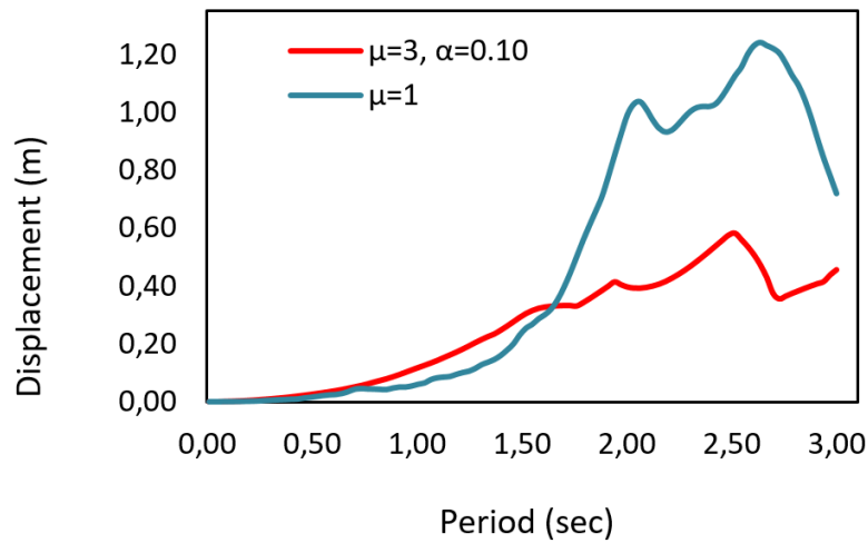
Figure 4 Elastic and inelastic displacement spectra.
