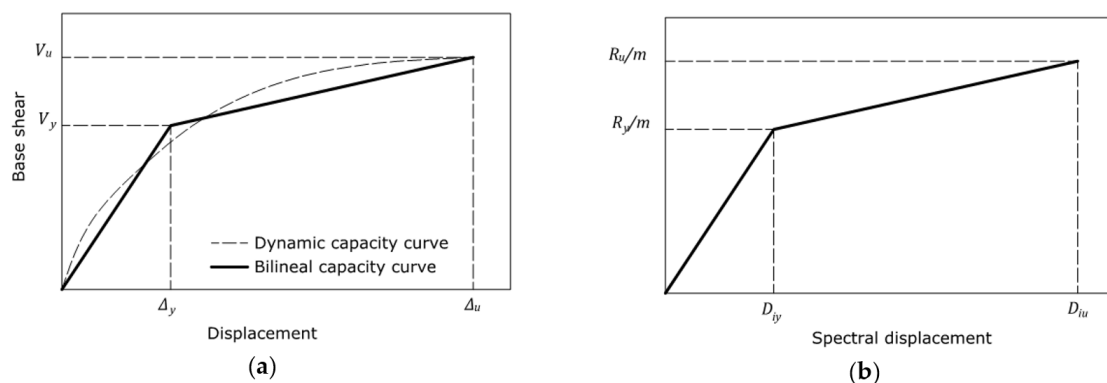
Figure 1 Illustration of the capacity curve of a structure and the behavior curve of the corresponding reference SDOF system as those used by the design method proposed: (a) Capacity curve, real and its bilinear approximation, (b) Approximate behavior curve in the ADRS format.
