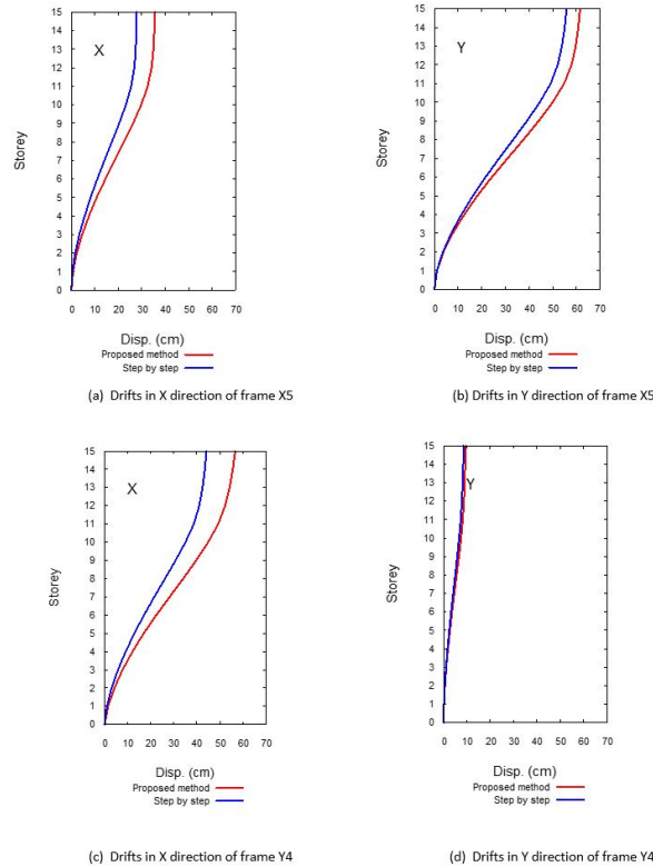
Figure 10 Comparison of the profile of maximum horizontal displacements for 15-story building.
