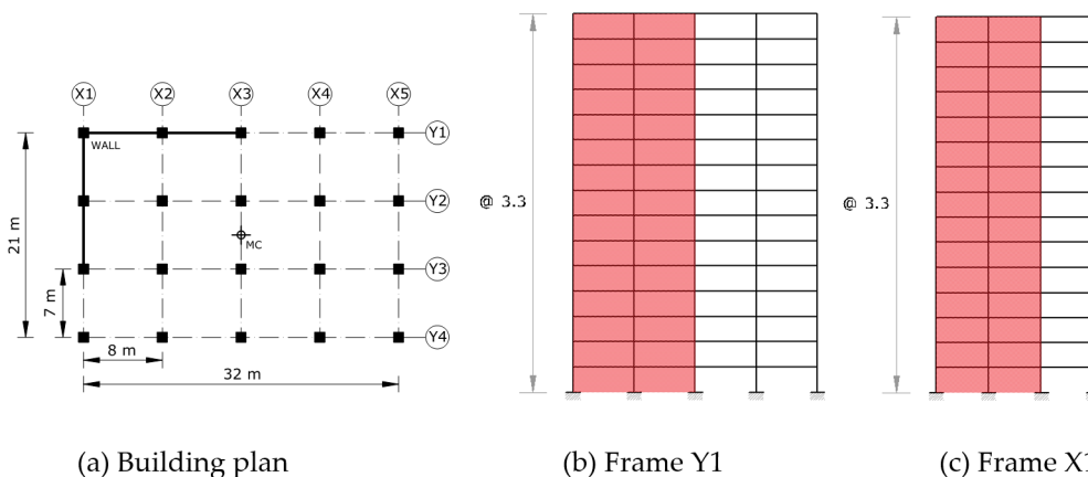
Figure 6 15-story building.
