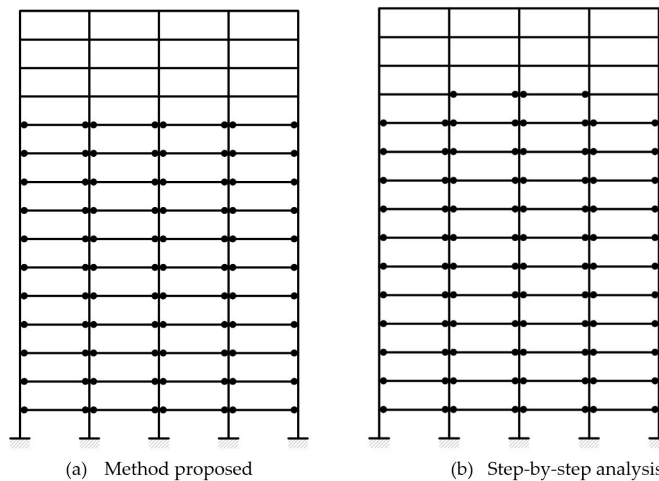
Figure 8 Damage distribution in frame X5 of the 15-story building.
