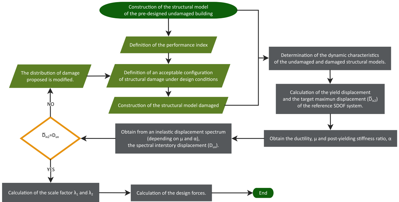
Figure 5 Flowchart of the displacement-based seismic design method with damage control.
