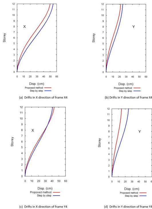
Figure 11 Comparison of the profile of maximum horizontal displacements for 12-story building.
