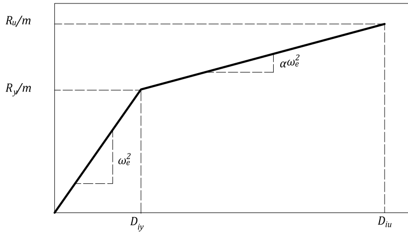
Figure 3 Behavior curve of a reference SDOF system.
