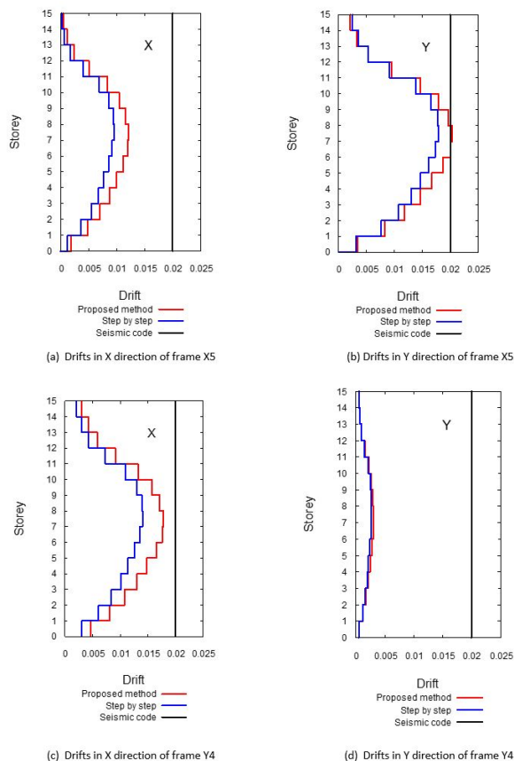
Figure 12 Comparison of the interstory drifts for 15-story building.
