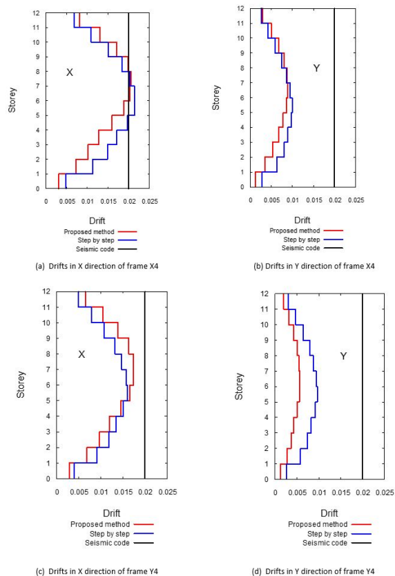
Figure 13 Comparison of the interstory drifts for 12-story building.
